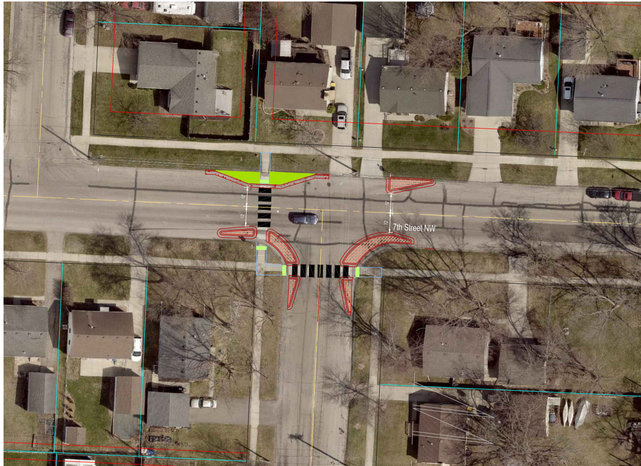
Concrete curb and gutter bump outs with pedestrian ramp access.
