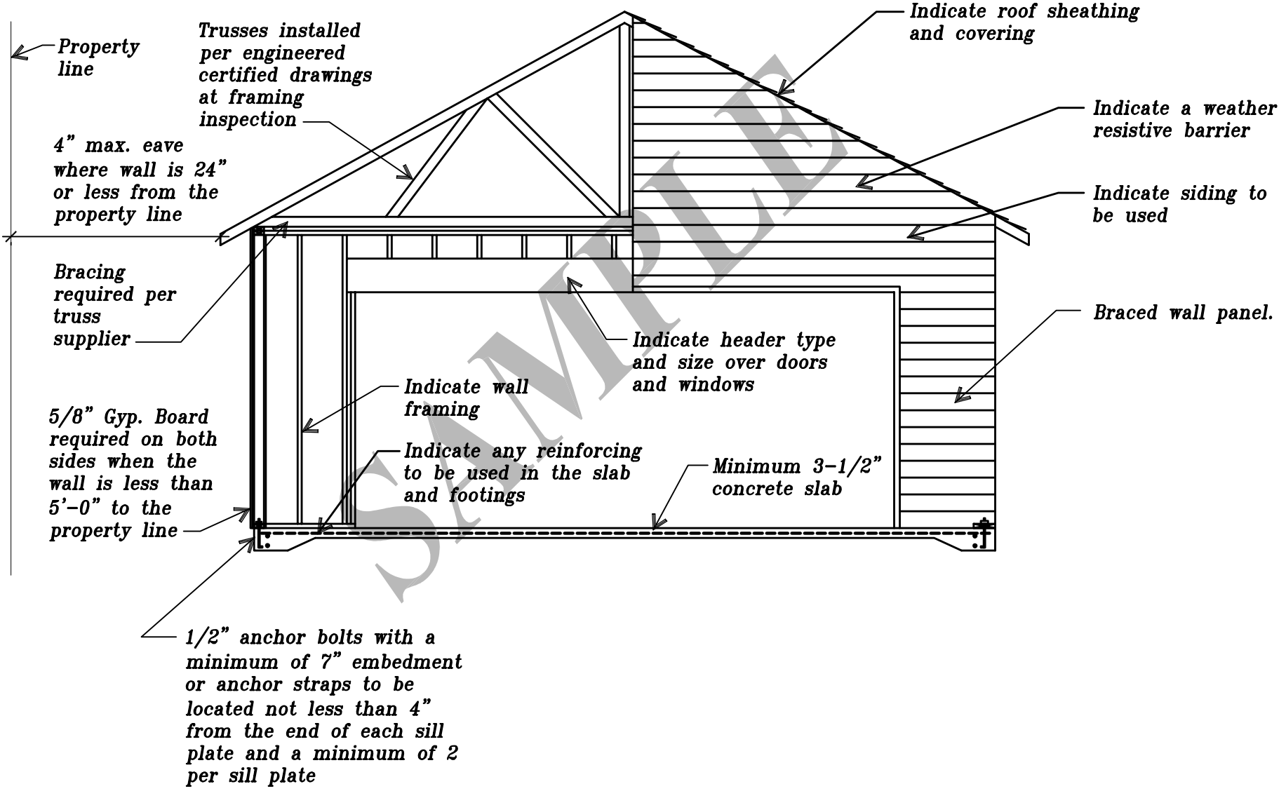
SECTION \ ELEVATION
