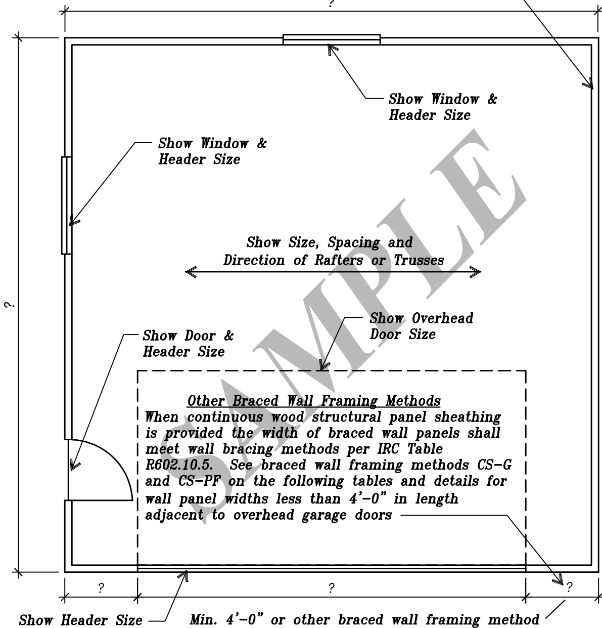
FLOOR PLAN
